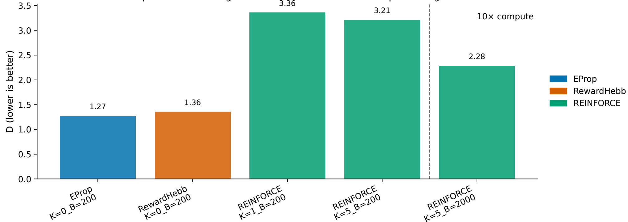
Compute fairness: alignment under matched forward-pass budgets
