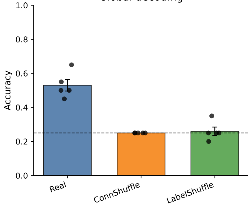
Global decoding
