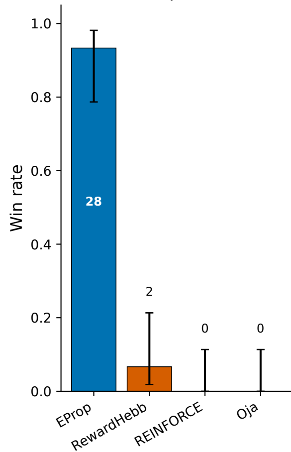
Best rule per patch (n=30 patches)
