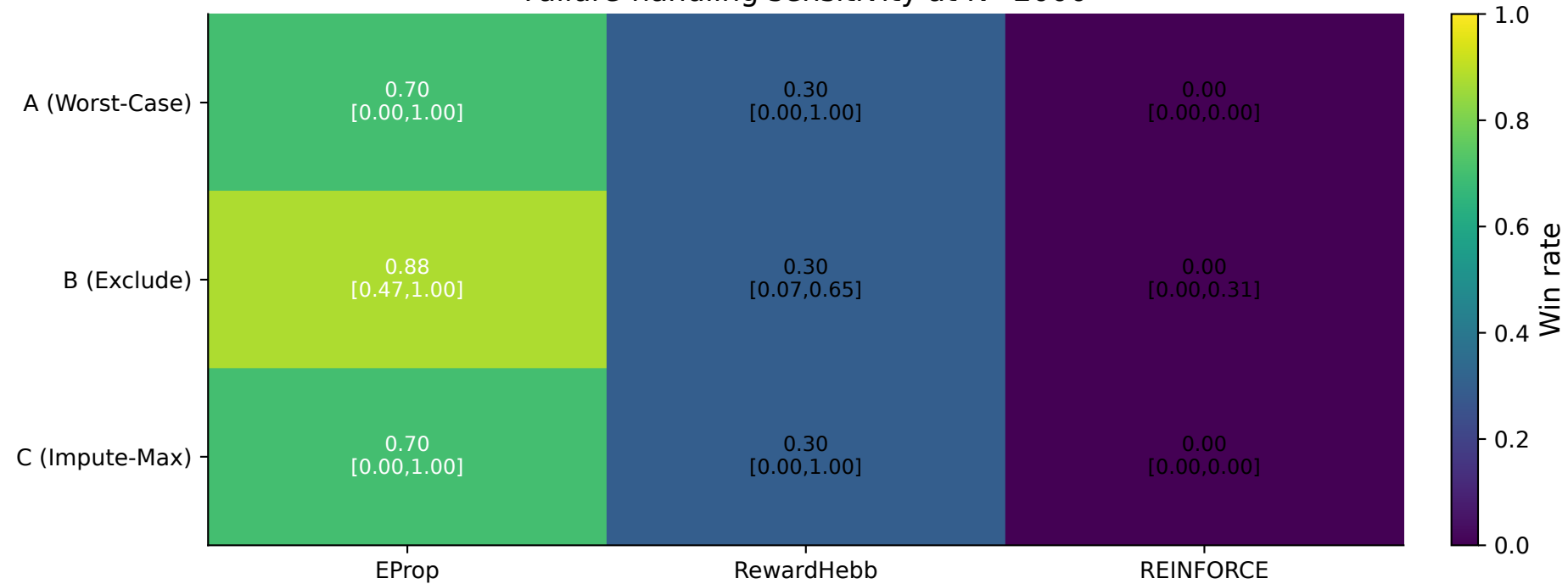
Failure-handling sensitivity at N=2000
