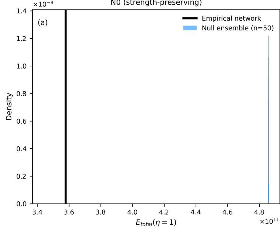
N0 (strength-preserving)
