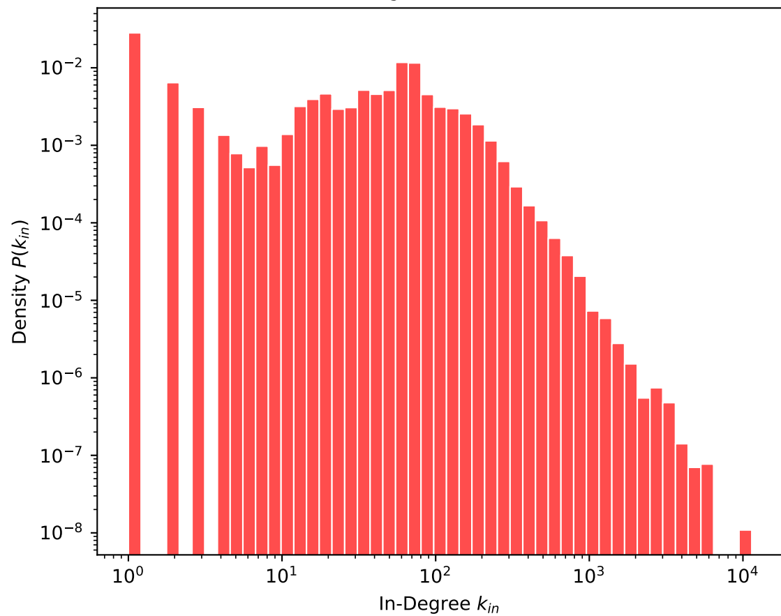
In-Degree Distribution
