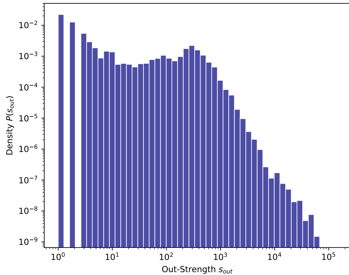
Out-Strength Distribution
