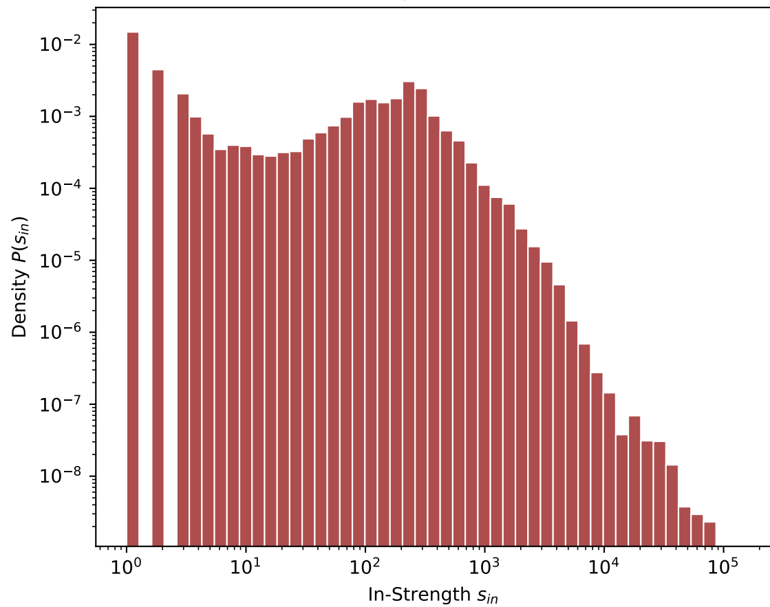
In-Strength Distribution
