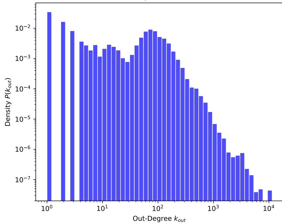
Out-Degree Distribution
