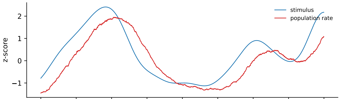
Switching variance
