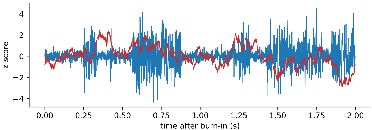
Switching variance
