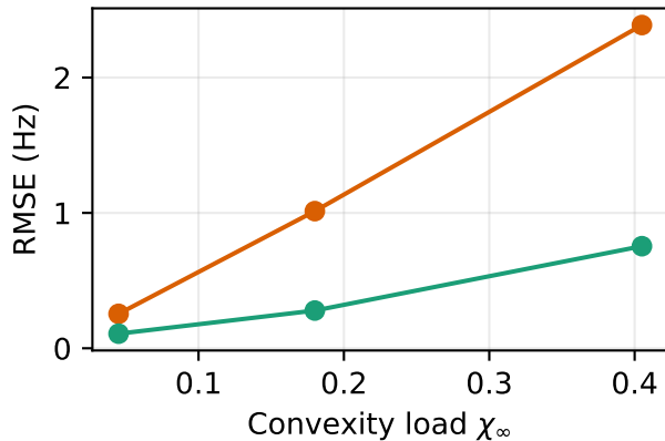
(b) Correction benefit and limit
