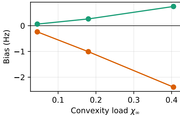
(a) Bias growth
