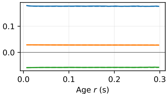
(a) Joint cumulant terms
