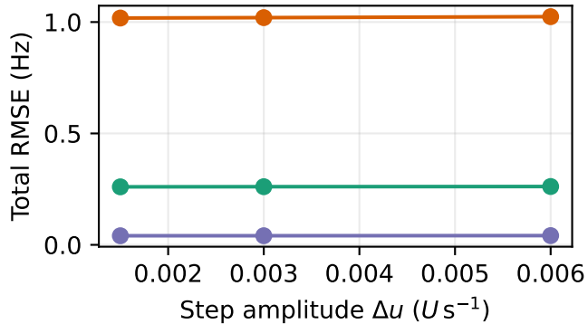
(b) Generalization across step size
