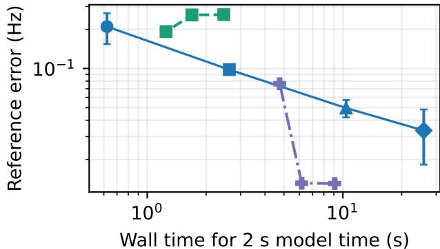
(a) Total accuracy--cost
