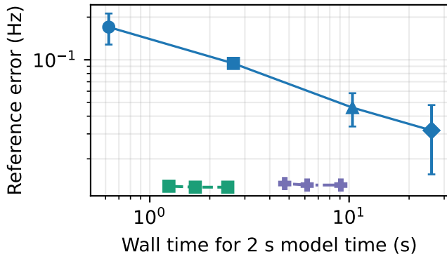
(b) Fluctuation accuracy--cost
