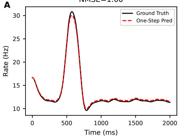
One-Step Prediction NMSE=1.00
