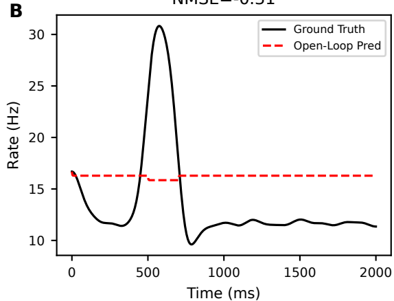
Open-Loop Rollout (Stable) NMSE=-0.31
