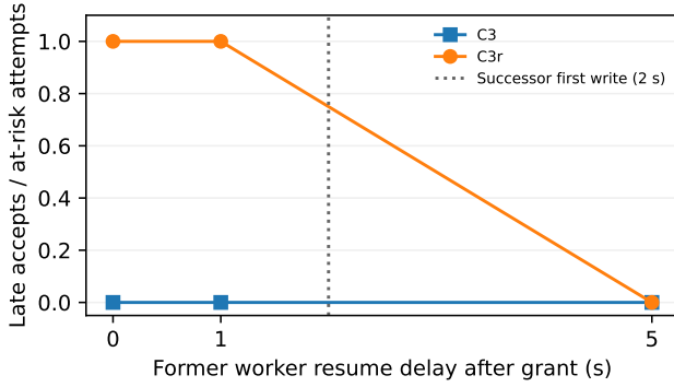
Fig. 5. Controlled after-grant late-accept fraction from raw trial rows. A dotted line marks the successor's first write at 2 s. This event-time schedule does not measure real cluster delay.
