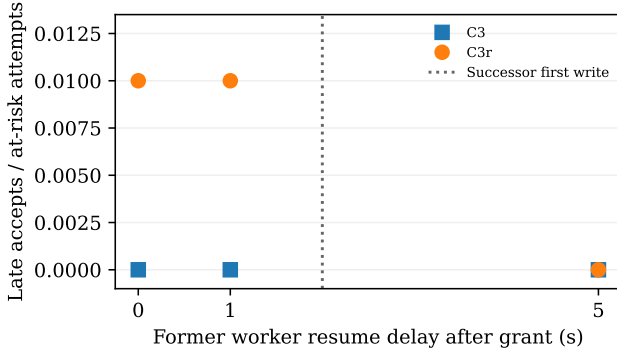
Fig. 5. Scripted after-grant late-accept fraction from raw trial rows. Markers represent the evaluated delays; the dotted line marks the scheduled successor first write. This is not a cluster timing measurement.
