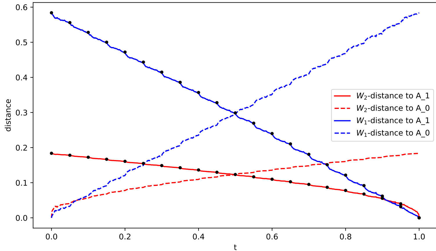
Wasserstein distance
