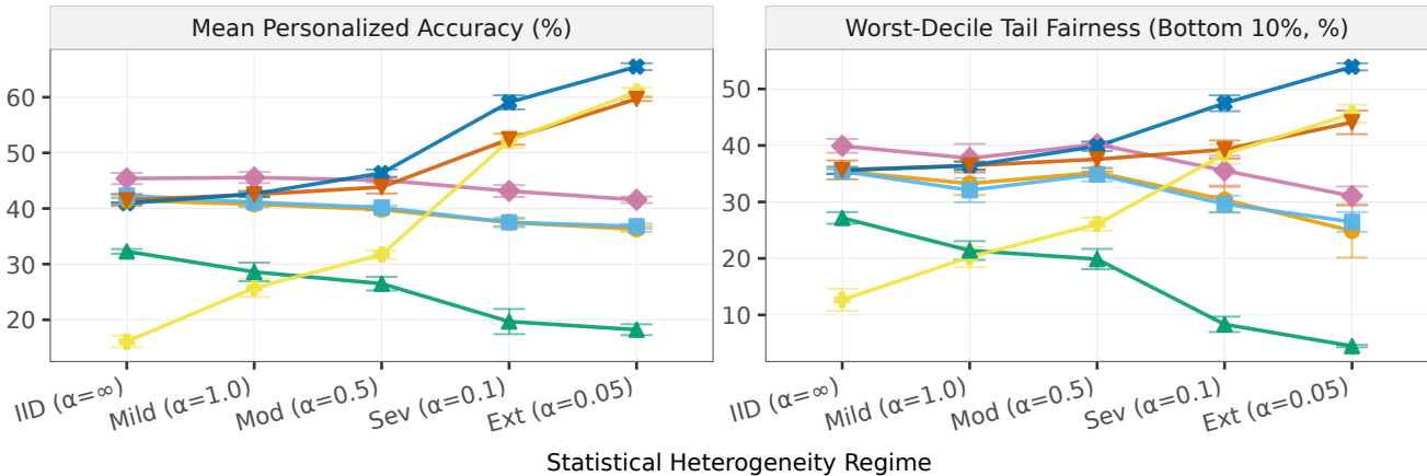
Accuracy / Fairness (%)
