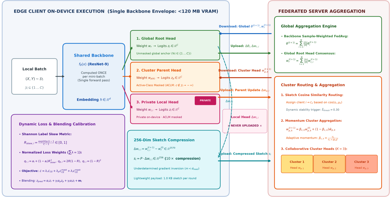
Fig. 2: Hierarchical Ensemble Personalization (HEP) System Architecture. Edge Client Execution (Left): A single forward pass on the shared convolutional backbone f_\theta(x) produces intermediate embeddings h \in \mathbb{R}^d , which are concurrently evaluated by three lightweight classification heads: (1) unmasked Global Root Head w_r , (2) cluster-collaborative Parent Head w_{p(k)} with Active-Class Logit Masking (ACLM), and (3) private Local Head w_{l,i} (which remains strictly on-device and is never uploaded). Dynamic loss weighting and inference logit blending are dynamically modulated by the Shannon entropy label skew metric R_{skew,i} . For cluster routing, linear Root-head updates \Delta w_{r,i} are projected into a 256-dimensional random sketch ( s_i = P \Delta w_{r,i} ), ensuring severe underdetermined gradient inversion ( m = 256 < d_{head} = 2570 ). Server Aggregation (Right): Backbones and Root heads undergo sample-weighted FedAvg, while compressed sketches drive cosine similarity cluster routing and momentum-updated Parent heads.
