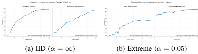
Fig. 3: Communication Round Convergence Trajectory on CIFAR-10 ResNet9 . Panel A: Under uniform IID data, Shannon entropy calibration shifts inference trust to the Root head, maintaining 71.03% personalized accuracy (72.73% global root consensus). Panel B: Under extreme Non-IID skew ( \alpha = 0.05 ), HEP rapidly ascends to 88.80% personalized accuracy, surpassing Ditto (87.87%), FedRep (87.07%), and FedAvg (57.53%).
