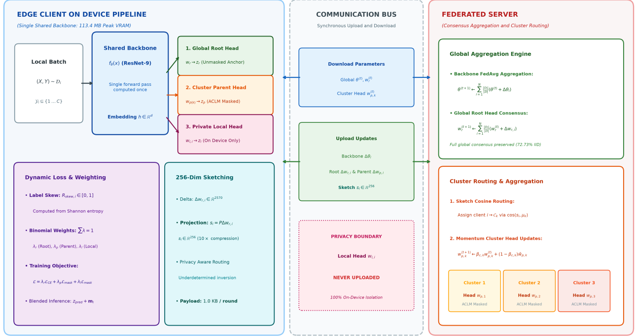
Fig. 2: Hierarchical Ensemble Personalization (HEP) System Architecture. Edge Client Execution (Left): A single forward pass on the shared convolutional backbone f_\theta(x) produces intermediate embeddings h \in \mathbb{R}^d , which are concurrently evaluated by three lightweight classification heads: (1) unmasked Global Root Head w_r , (2) cluster-collaborative Parent Head w_{p(k)} with Active-Class Logit Masking (ACLM), and (3) private Local Head w_{l,i} (which remains strictly on-device and is never uploaded). Dynamic loss weighting and inference logit blending are dynamically modulated by the Shannon entropy label skew metric R_{skew,i} . For cluster routing, linear Root-head updates \Delta w_{r,i} are projected into a 256-dimensional random sketch ( s_i = P\Delta w_{r,i} ), ensuring severe underdetermined gradient inversion ( m = 256 < d_{head} = 2570 ). Server Aggregation (Right): Backbones and Root heads undergo sample-weighted FedAvg, while compressed sketches drive cosine similarity cluster routing and momentum-updated Parent heads.
