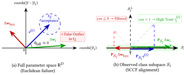
Figure 2: Geometric Intuition of Subspace-Constrained Cosine Filtering (SCCF). (a) In full parameter space \mathbb{R}^D , an honest client with non-IID label skew ( y_i \subset \mathcal{Y} ) updates primarily along active coordinates \text{coords}(y_i) , creating large Euclidean distance to consensus \mathbf{c}^{(t)} and triggering false rejection. (b) Projecting via \mathbf{P}_{S_i} onto active subspace S_i removes unobserved dimensions: honest updates align with consensus ( \cos \approx 1 , high trust \tau_i^{(t)} ), while Byzantine attacks remain separated.
