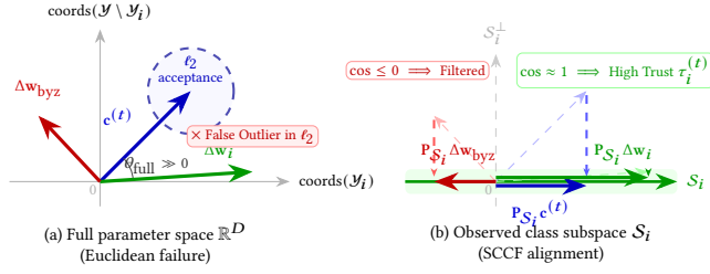
Figure 2: Geometric Intuition of Subspace-Constrained Cosine Filtering (SCCF). (a) In full parameter space \mathbb{R}^D , an honest client with non-IID label skew ( \mathcal{Y}_i \subset \mathcal{Y} ) updates primarily along active coordinates \text{coords}(\mathcal{Y}_i) , creating large Euclidean distance to consensus \mathbf{c}^{(t)} and triggering false rejection. (b) Projecting via \mathbf{P}_{S_i} onto active subspace S_i removes unobserved dimensions: honest updates align with consensus ( \cos \approx 1 , high trust \tau_i^{(t)} ), while Byzantine attacks remain separated.
