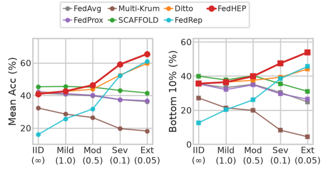
Figure 4: CIFAR-100 Personalization and Tail Fairness. Mean test accuracy (left) and bottom-10% tail fairness (right) across Dirichlet skew regimes on 100-class CIFAR-100.
