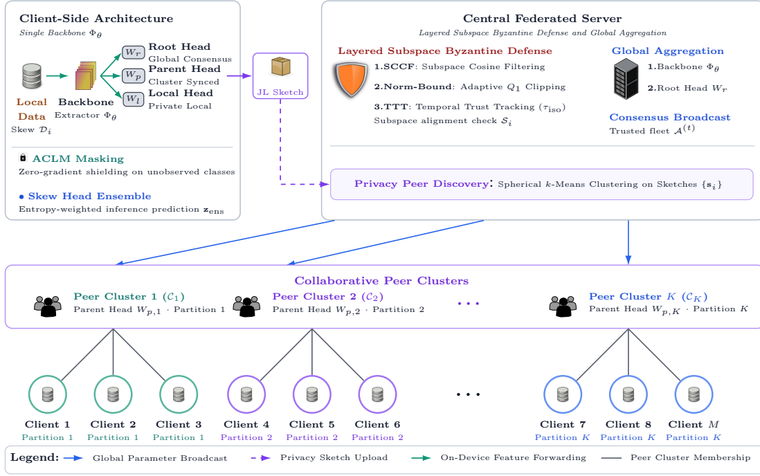
Figure 1: Overview of FedHEP Architecture. (Left) On-device client with a single backbone, tripartite head ensemble. (Right) Server-side sketch clustering and layered subspace defense.
