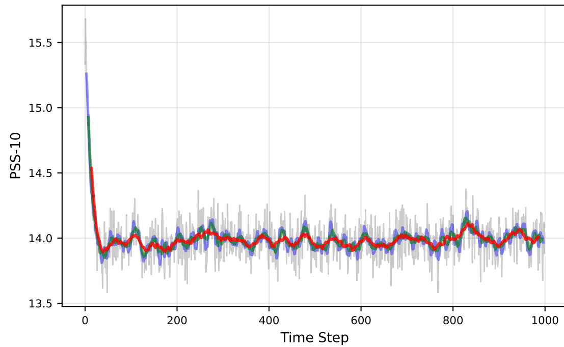
PSS-10
