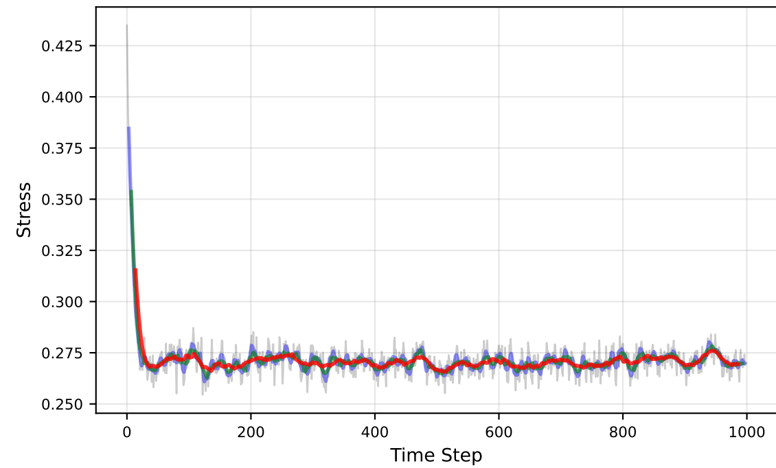
Stress
