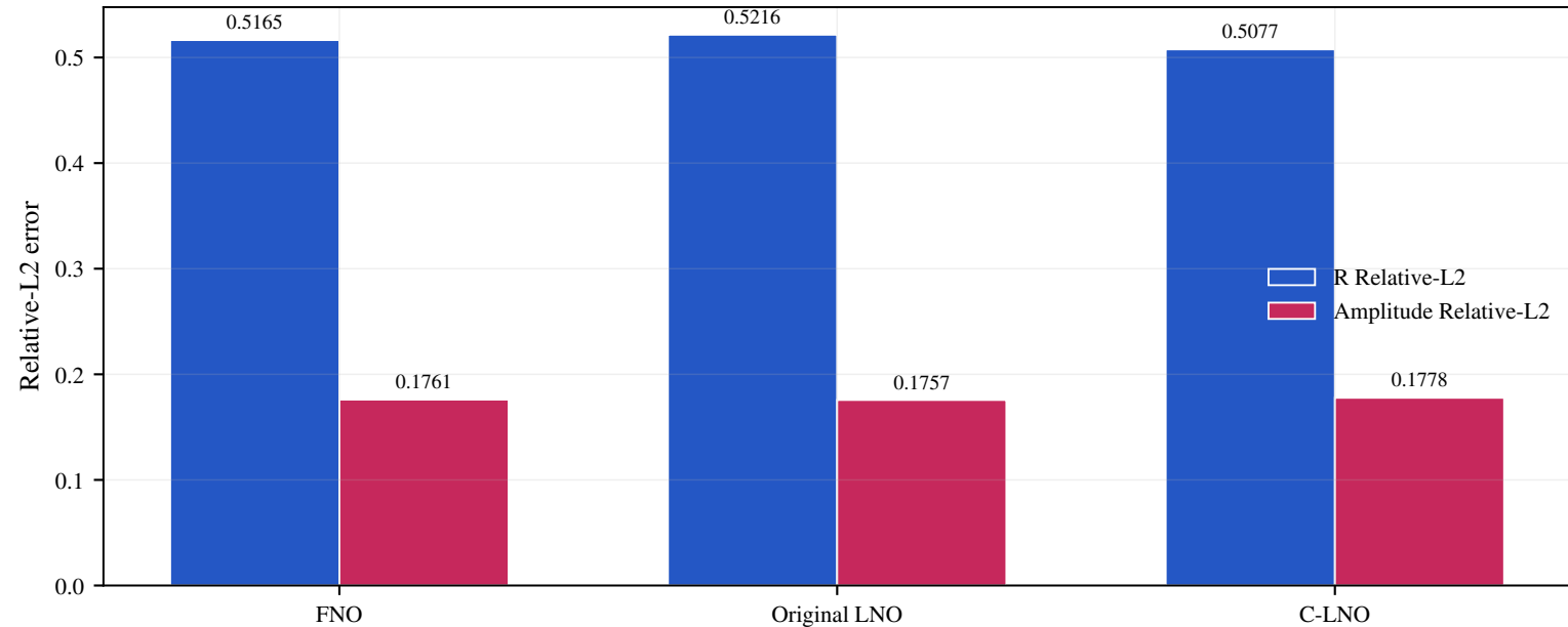
Overall One-Step Reconstruction Accuracy
