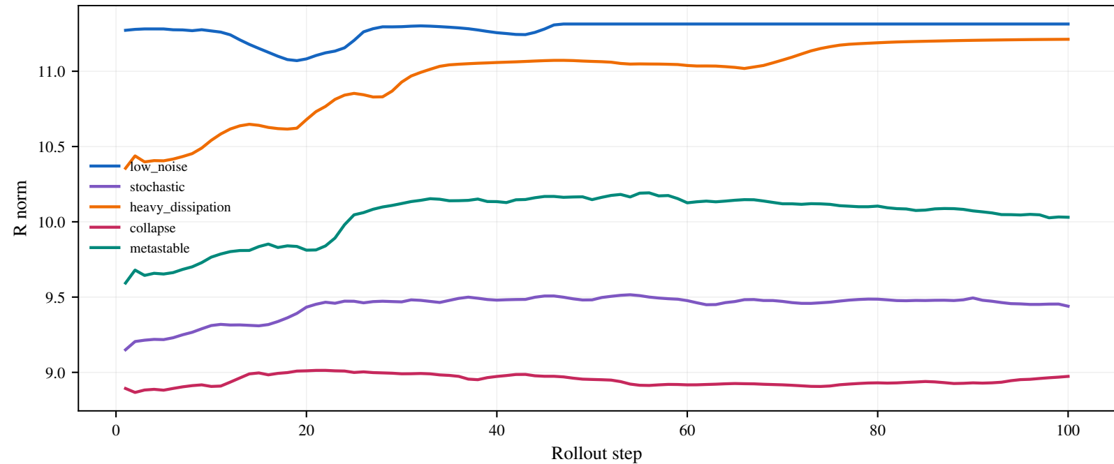
C-LNO Long-Horizon R-Norm Stability
