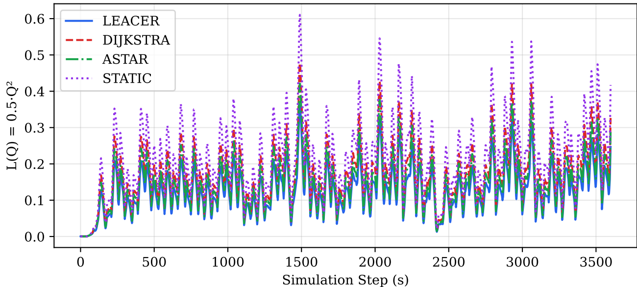
Fig. 12 — Lyapunov Drift L(Q) — Queue Stability
