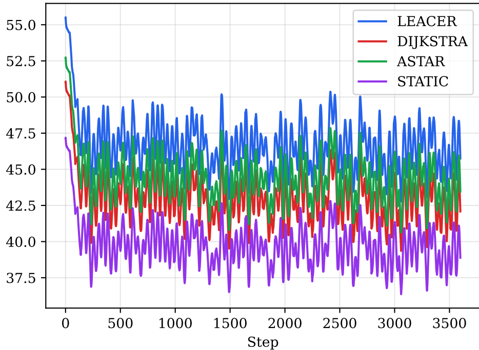
Fig. 7a — Speed (Rush Hour)
