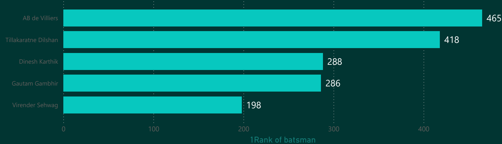
1Rank of batsman by fullName
