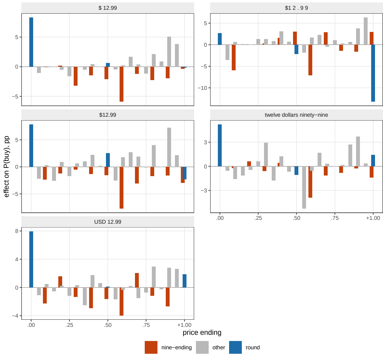
E6 (Number formatting): the ending profile
