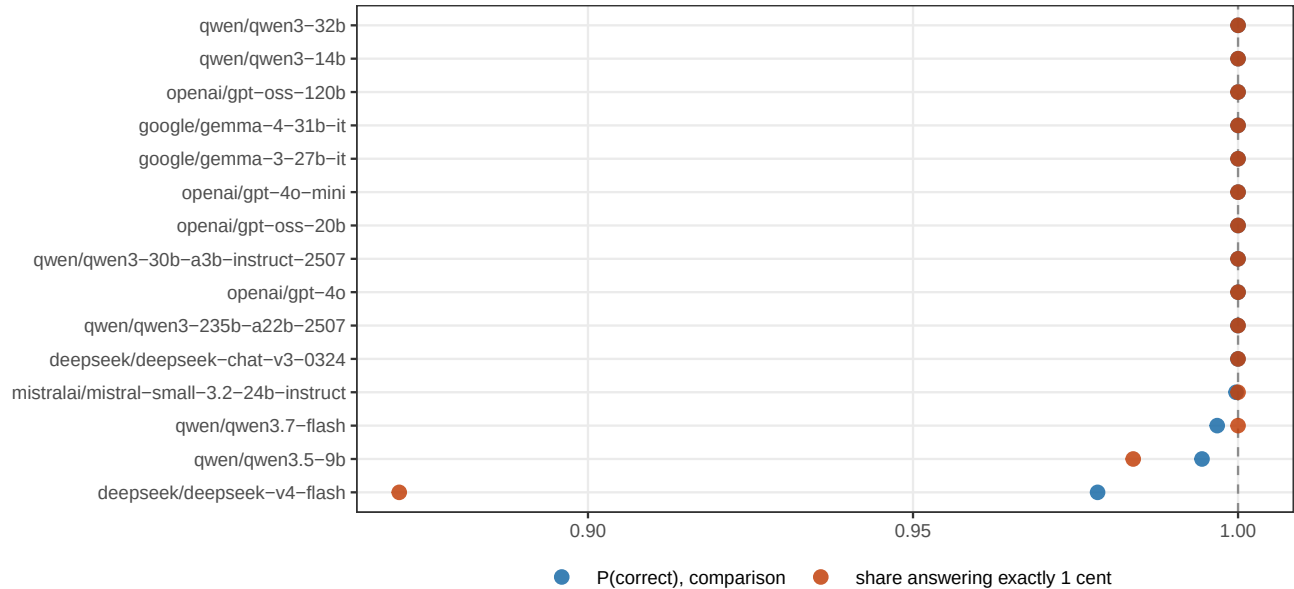
E9: accuracy on the arithmetic probes
