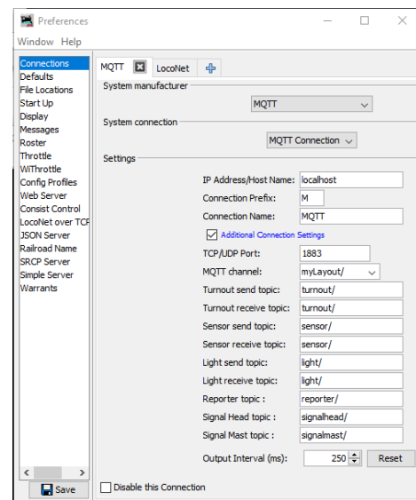
JMRI Connections (v 4.21.2)
