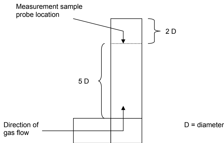
Figure 4-2: Position of sampling probe location
