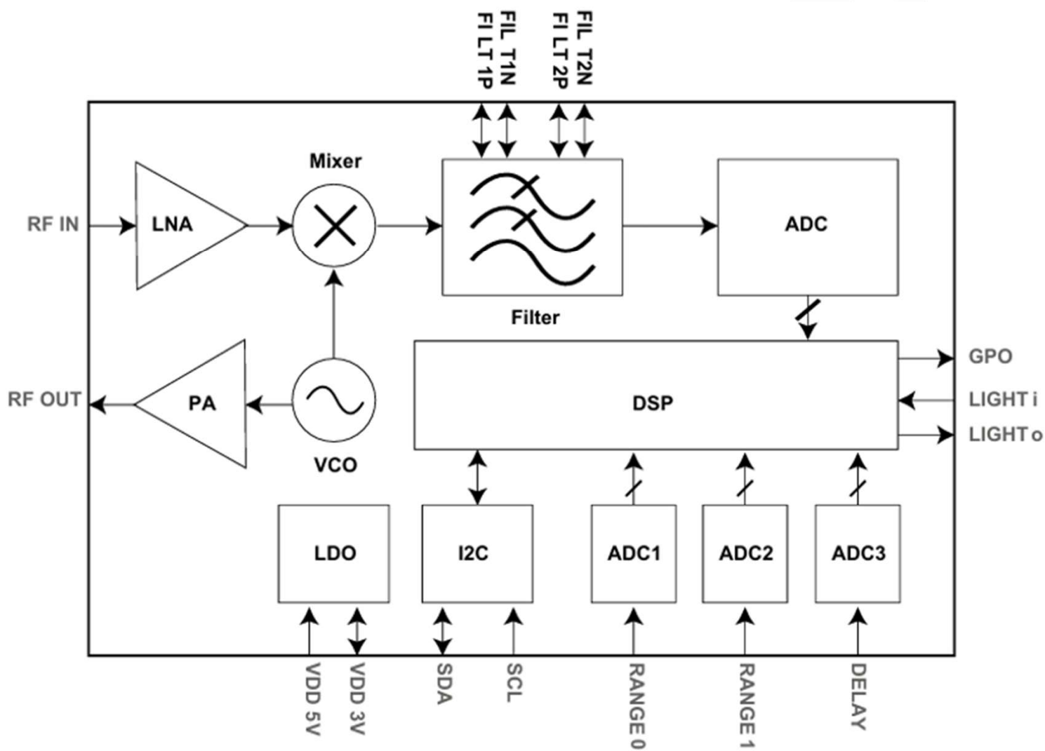
Figure : KW007 Block Diagram
