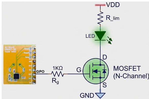
* LED driver circuit with pin GPO.
