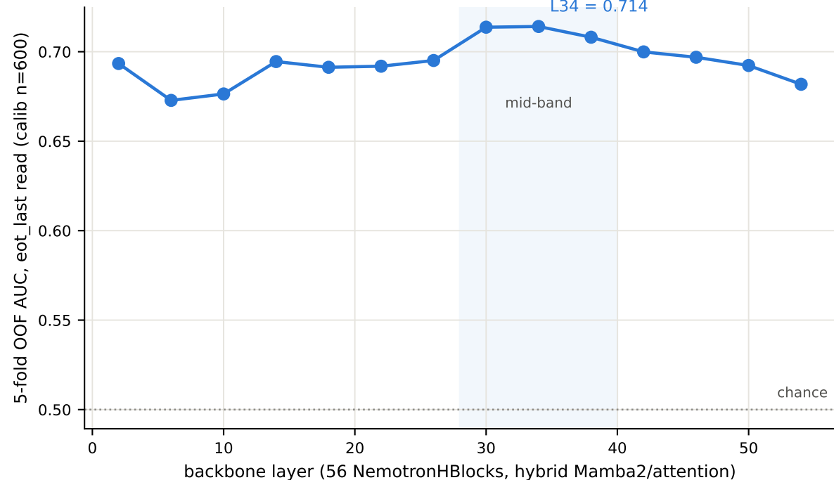
Second duplex family, same probe recipe — NemotronLabs-VoiceChat-11B layer sweep replicates the mid-band structure (MiniCPM-o: L22/28)
