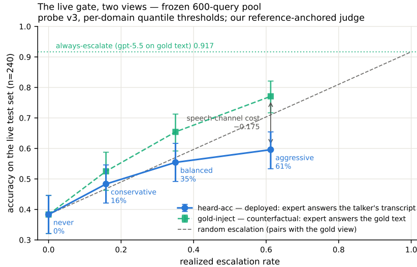
Figure 15: Dual-view live tradeoff, full pool ( n=240 ); companion to Figure 11.
