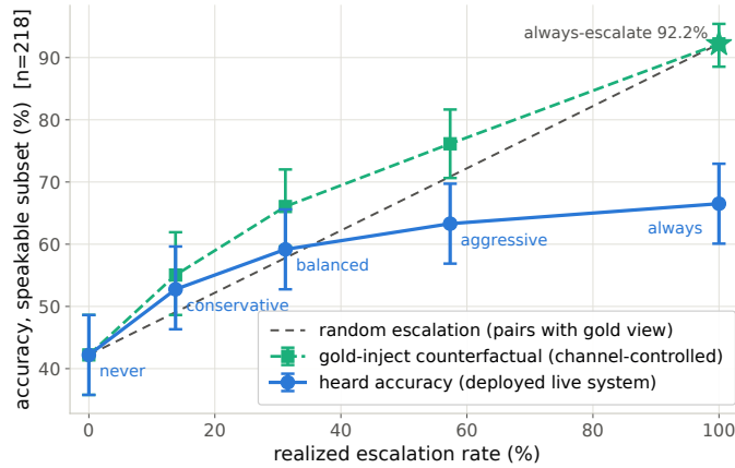
Figure 11: Live dual-view tradeoff ( n=218 speakable subset). Blue: honest heard accuracy of the live system (paired-bootstrap CIs). Green: the channel-controlled counterfactual (same sessions, escalated rows re-scored with gold-text expert answers) with its paired random reference (dashed). The view-to-view gap is the speech-channel price; the floor-to-floor gap to offline operation is the audio + streaming-answer tax.
