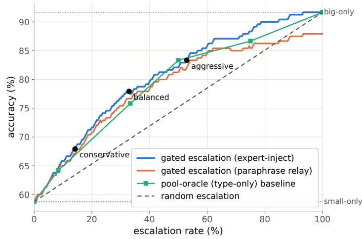
Figure 6: Accuracy vs. escalation rate, frozen test split: gated escalation vs. random-escalation and pool-oracle (type-only) baselines between the small-only and big-only endpoints.
