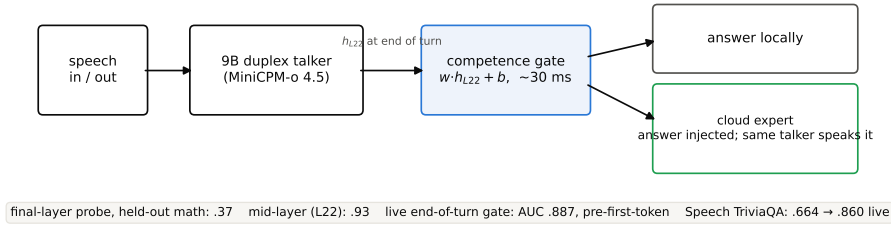
Figure 1: The system and the headline numbers. A linear read of the talker’s mid-network hidden state at end of turn decides, before decoding starts, whether the talker answers or a cloud expert does — and the expert’s answer is spoken by the same talker, preserving the session.
