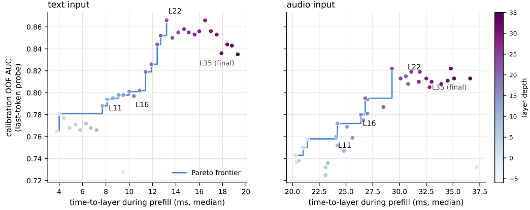
Figure 11: Fork-depth Pareto: per-layer wall-time vs. gate quality.
