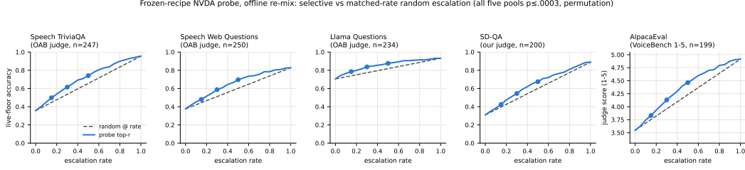
Figure 5: Re-mix curves for the frozen-recipe NVDA probe: selective (top- r by probe score) vs. matched-rate random on the five transfer pools, official judge per pool. Every pool separates, including the three that are flat on MiniCPM.
