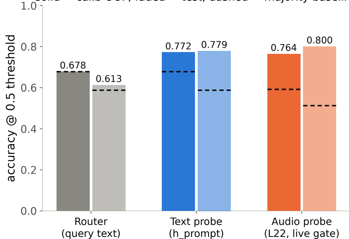
(a) Accuracy on our eval splits
