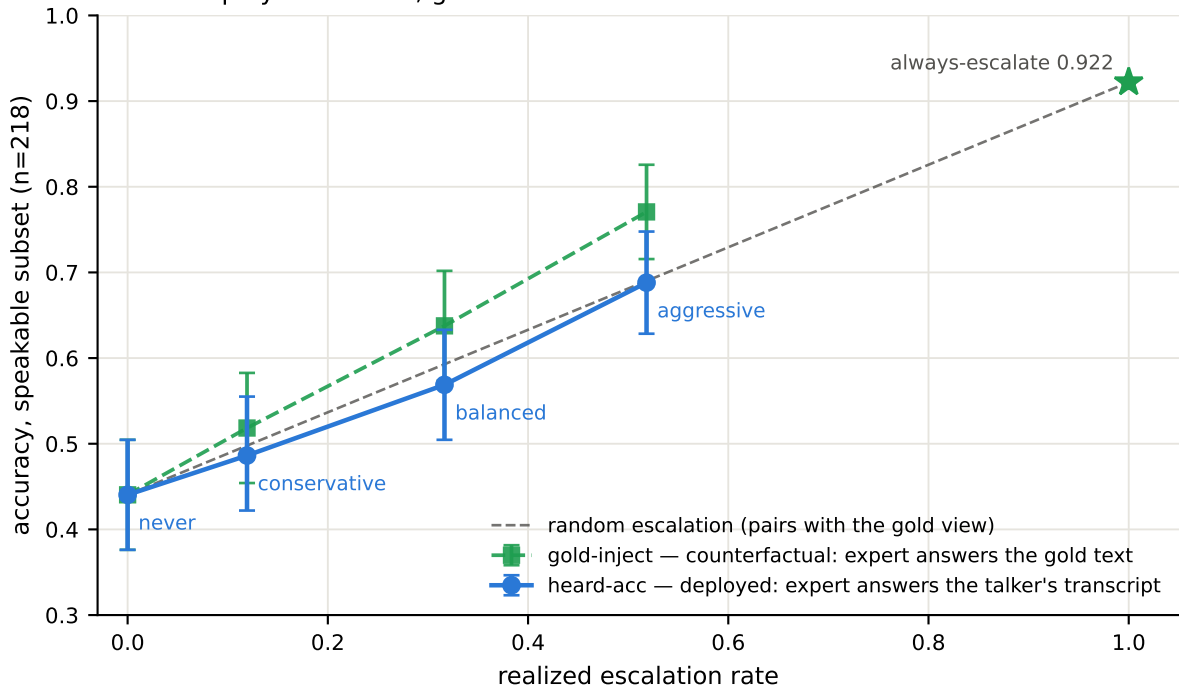
Accuracy vs escalation rate — speakable subset (“TTS-fair” view) blue = deployed channel, green = channel-controlled counterfactual
