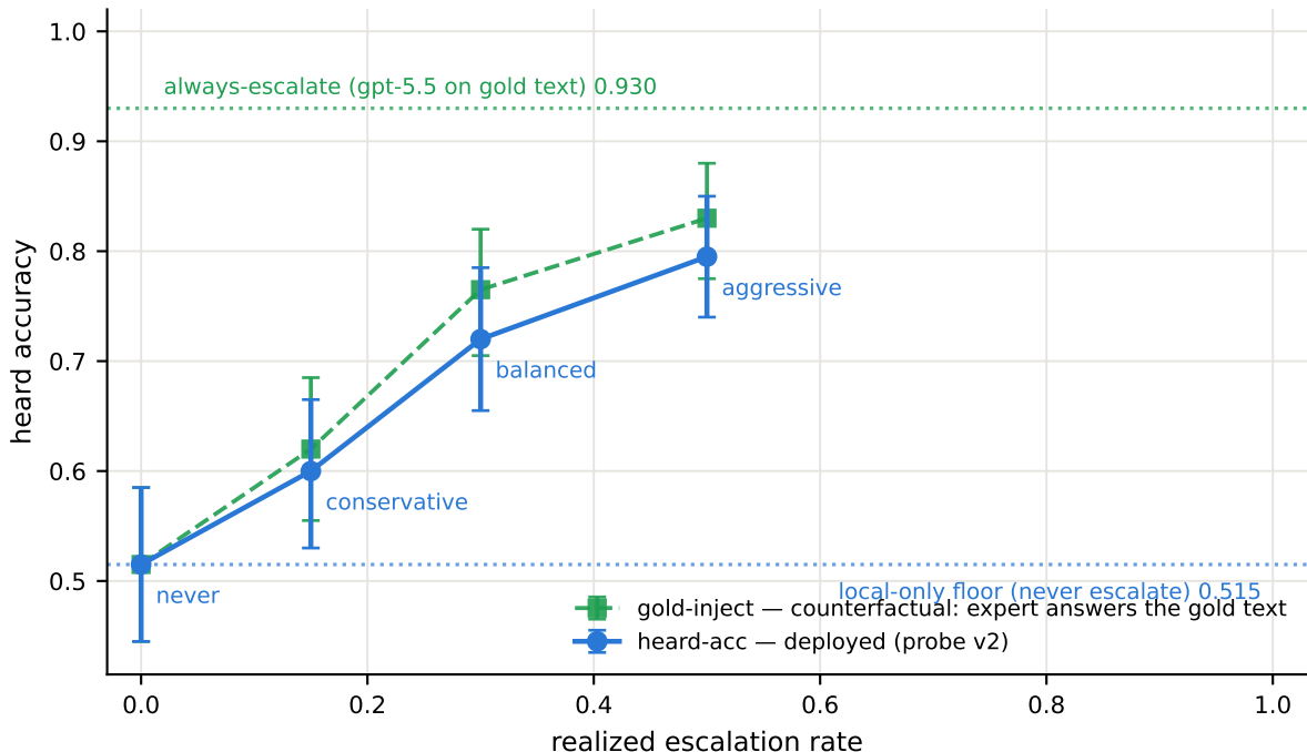
Accuracy vs escalation rate — SD-QA — real human speech (VoiceBench, n=200) probe v2, per-domain quantile thresholds; our reference-anchored judge
