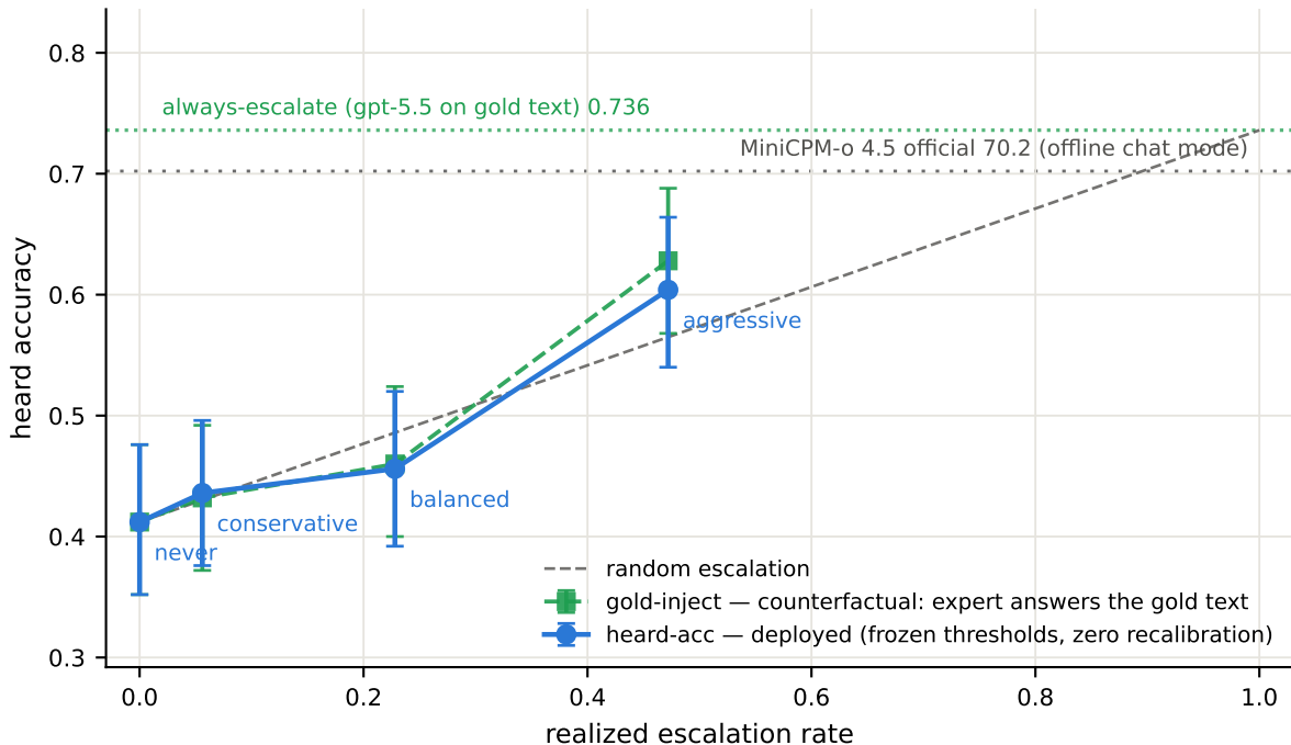
Accuracy vs escalation rate — Speech Web Questions (OpenAudioBench, n=250) gate + thresholds frozen from the 600-query calibration pool
