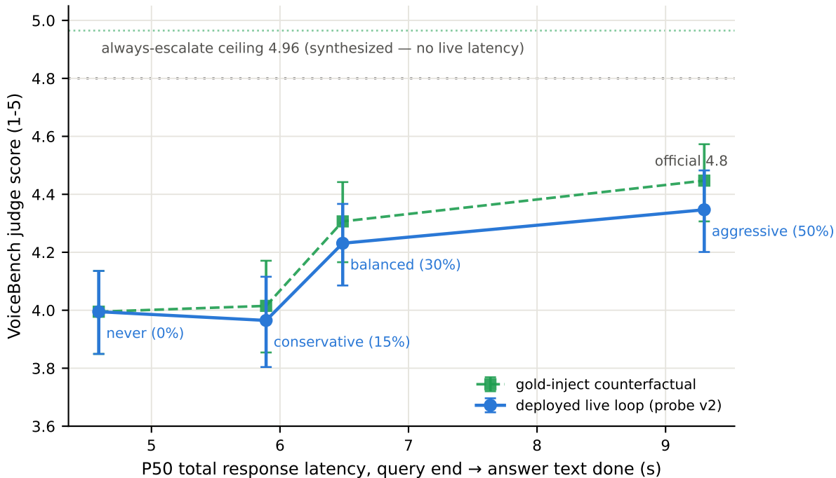
What latency buys — VoiceBench AlpacaEval (n=199) probe v2, per-domain quantile thresholds; VoiceBench's own gpt-4o-mini judge prompt (1-5)
