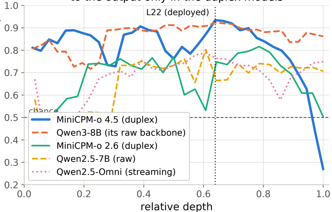
B. The distributed part of the read decays to the output only in the duplex models
