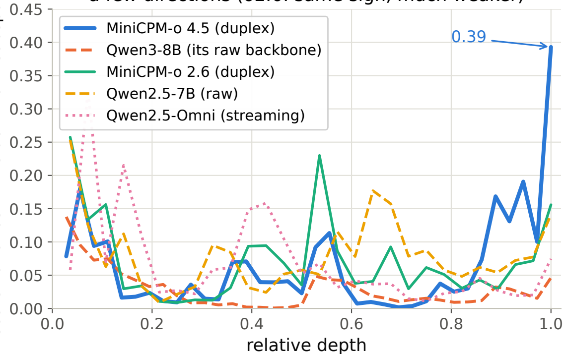
A. At the output the o4.5 read collapses onto a few directions (o2.6: same sign, much weaker)
