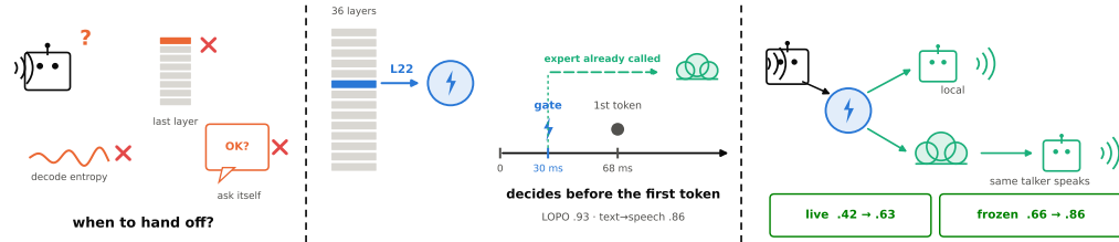
Figure 1: Left: standard competence readouts break on duplex models. Middle: a mid-network (L22) linear read decides in \sim 30 ms — before the first output token — so the expert call is already in flight while local decoding would just be starting. Right: the live system hands off mid-conversation and the same talker speaks the expert’s answer, improving real duplex sessions ( .422 \rightarrow .633 ) and, frozen, public speech benchmarks (Speech TriviaQA .664 \rightarrow .860 ).
