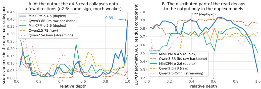
Figure 7: Non-destructive decomposition of the probe's held-out score at every depth. Left: share of score variance carried by the layer's five dominant directions. Right: transfer AUC of the residual (distributed) component — intact to the output on both raw backbones and on the omni-streaming control, decaying to inversion over the final layers of both duplex models.
