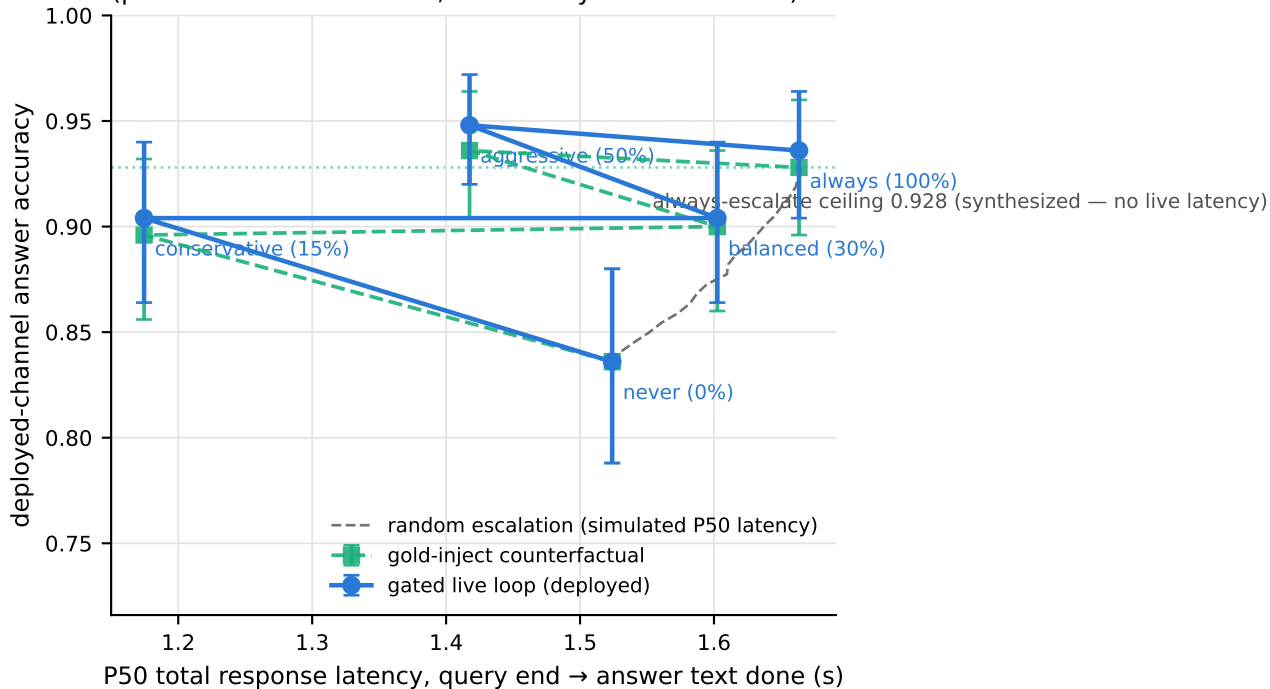
What latency buys — Speech Llama Questions (OpenAudioBench, n=250) (points = escalation arms, labelled by escalation rate)
