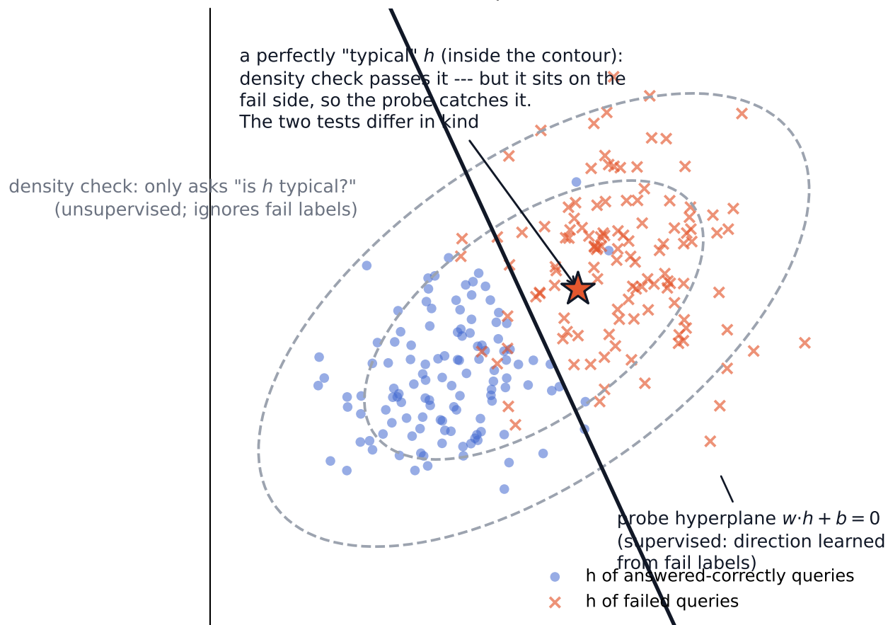
View 1: hidden-state space h (4096-d, drawn as 2-d)
