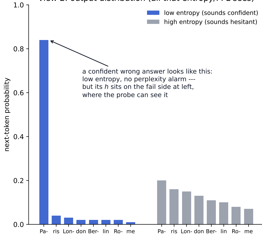
View 2: output distribution (all that entropy/PPL sees)
