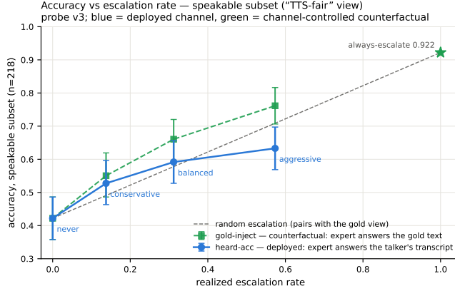
Figure 3: Live dual-view tradeoff ( n=218 speakable subset). Blue: honest heard accuracy of the live duplex system (paired-bootstrap CIs). Green: the channel-controlled counterfactual (same sessions, escalated rows re-scored with gold-text expert answers) with its paired random reference (dashed). The view-to-view gap is the speech-channel price; the floor-to-floor gap to offline operation is the audio + streaming-answer tax.
