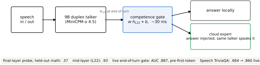
Figure 1: The system and the headline numbers. A linear read of the talker’s mid-network hidden state at end of turn decides, before decoding starts, whether the talker answers or a cloud expert does — and the expert’s answer is spoken by the same talker, preserving the session.
