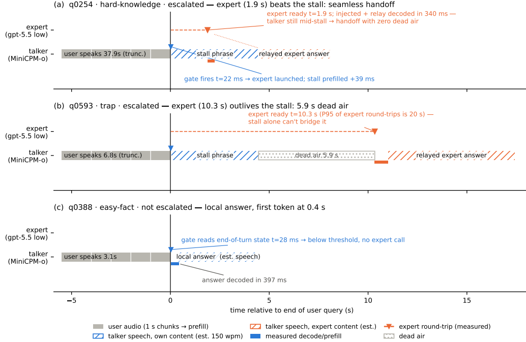
Figure 12: Three real sessions from recorded timers: expert beats the stall phrase (seamless); expert outlives it (dead air, the P99 signature); gate stays closed (first token 0.4 s).
