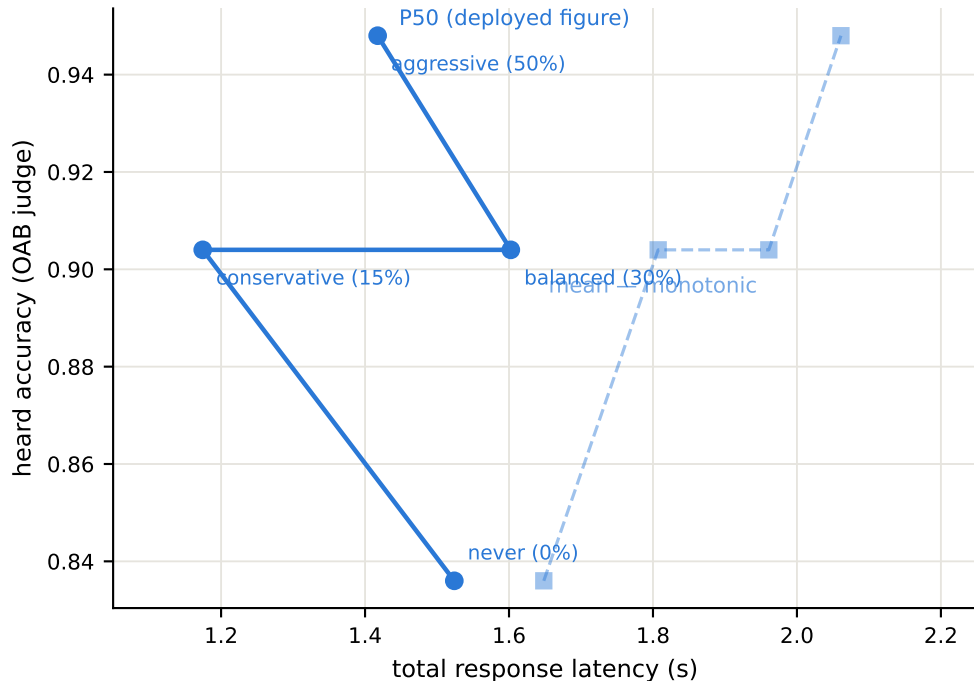
The left-fold lives only in the median — Llama Questions, same arms, two latency statistics
