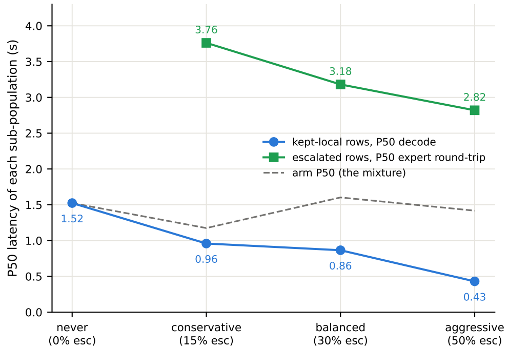
Why: the probe escalates the slowest local decodes — the kept-local median falls faster than the expert path enters
