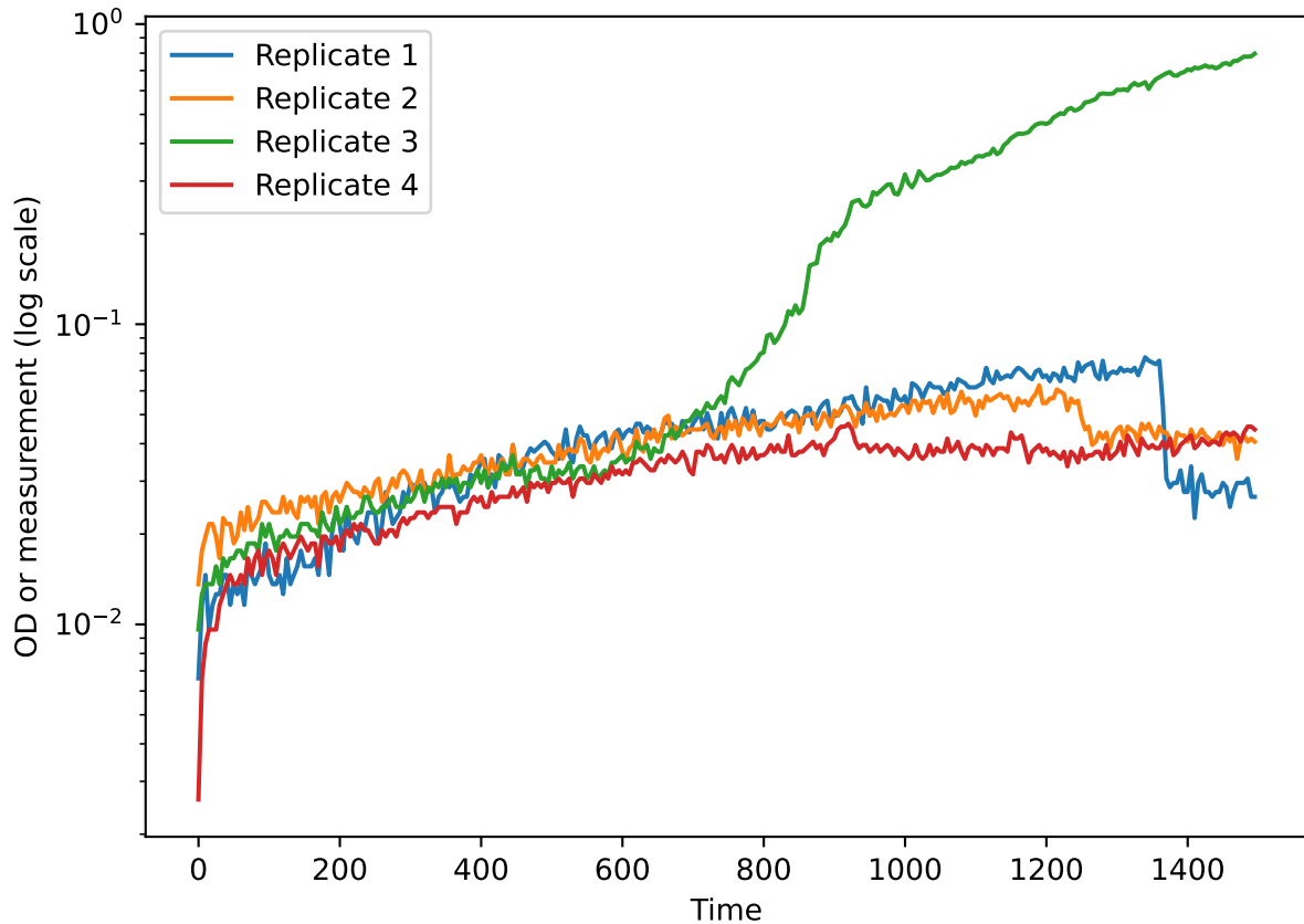
TB204 Cm=7 Growth Curves
